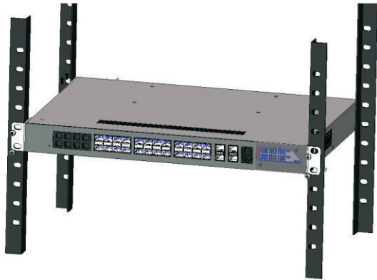
Figure 2-2 Install switch to the rack
